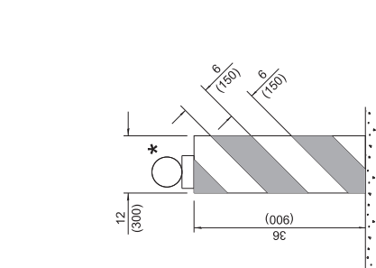
VERTICAL BARRICADE
