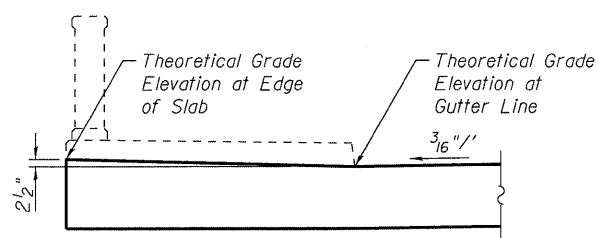
SIDEWALK DETAIL
