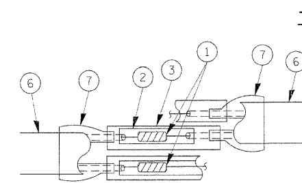
DETAIL "A" LOOP-TO-LOOP SPLICE
