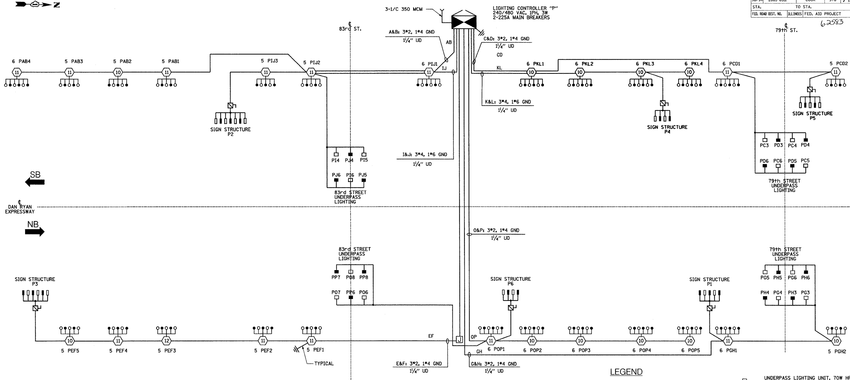
SINGLE LINE DIAGRAM LIGHTING CONTROLLER "P"
