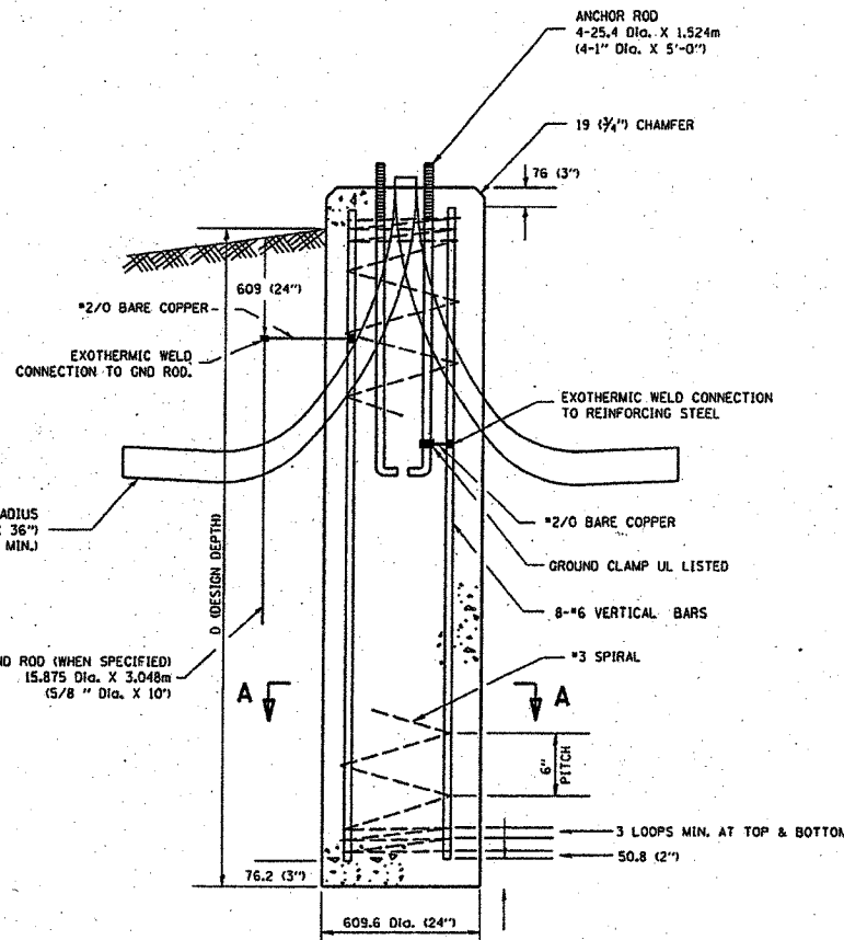
FOUNDATION DETAIL
