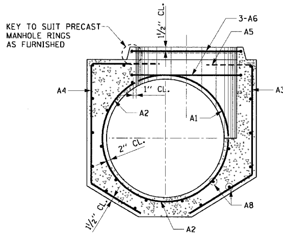
SECTION B-B MANHOLE BASE FOR SEWERS 36" DIA. AND 42" DIA.
