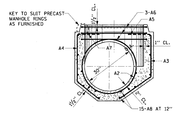
SECTION C-C MANHOLE BASE FOR 30" DIA. SEWERS
