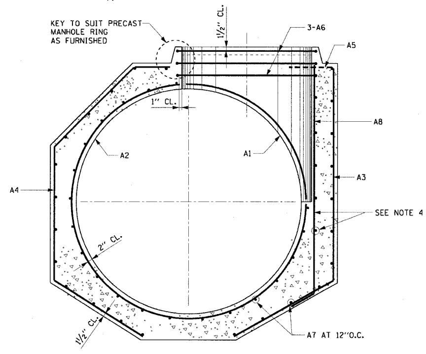
SECTION A-A MANHOLE BASE FOR SEWER 48" DIA. AND 120" DIA. INCLUSIVE
