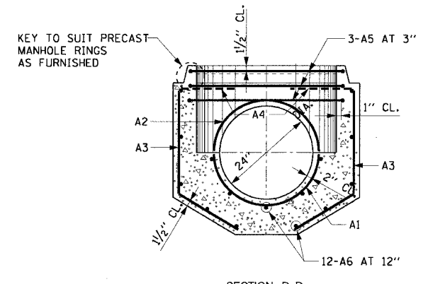
SECTION D-D MANHOLE BASE FOR 24" DIA. SEWERS
