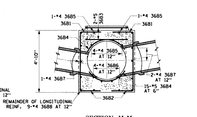
SECTION M-M 36" DIA. SEWER
