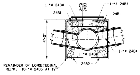
SECTION M-M
