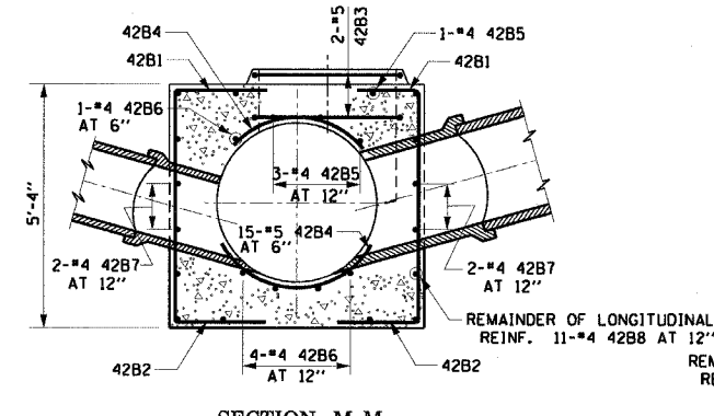
SECTION M-M 42" DIA. SEWER
