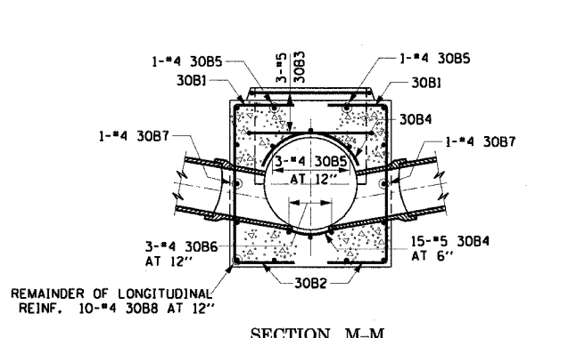
SECTION M-M 30" DIA. SEWER
