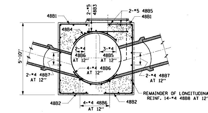
SECTION M-M 48" DIA. SEWER
