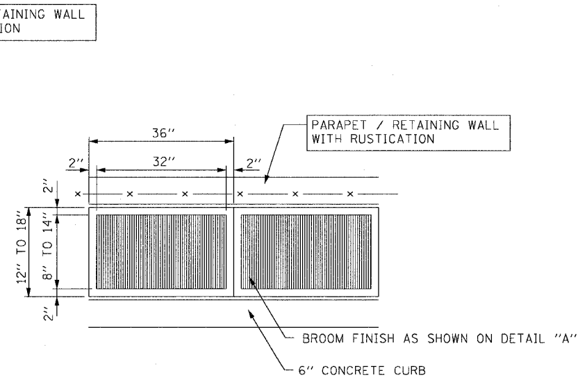
DETAIL "B" CALIFORNIA FINISH
