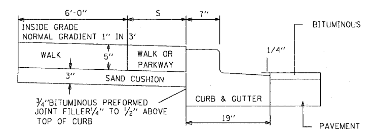
SECTION AT A-A
