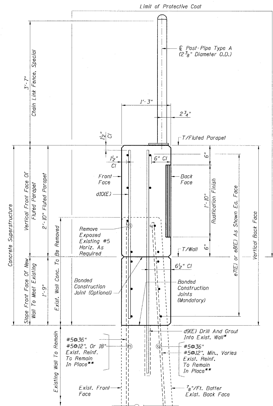
SECTION H-H 7/8" FT. BATTER EXISTING BACK FACE
