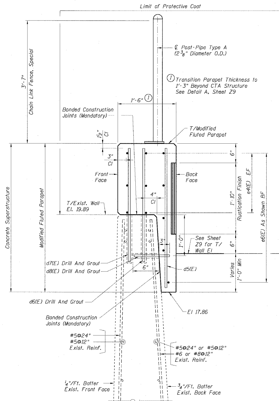
SECTION G-G
