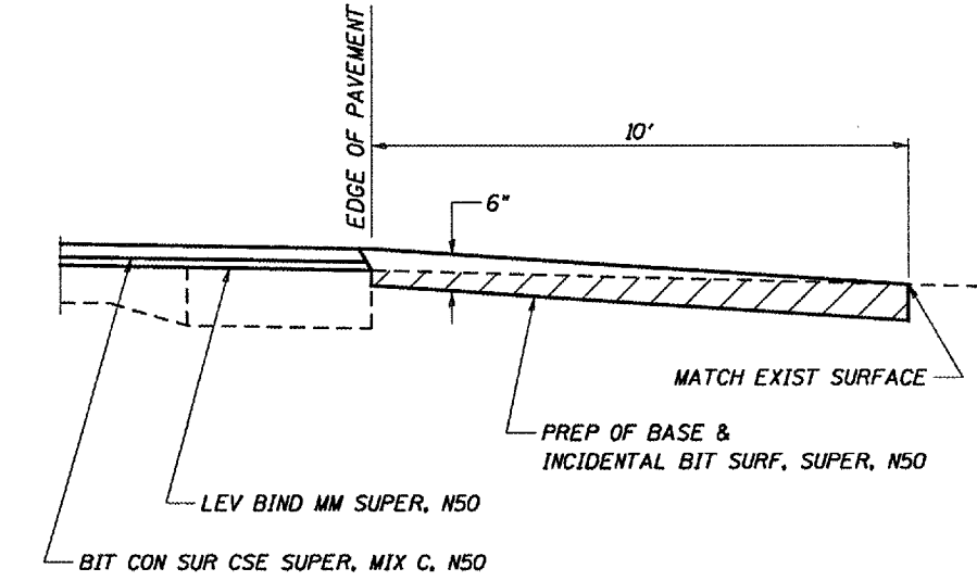
SECTION D-D FOR OIL & CHIP AND AGGREGATE SIDEROAD
