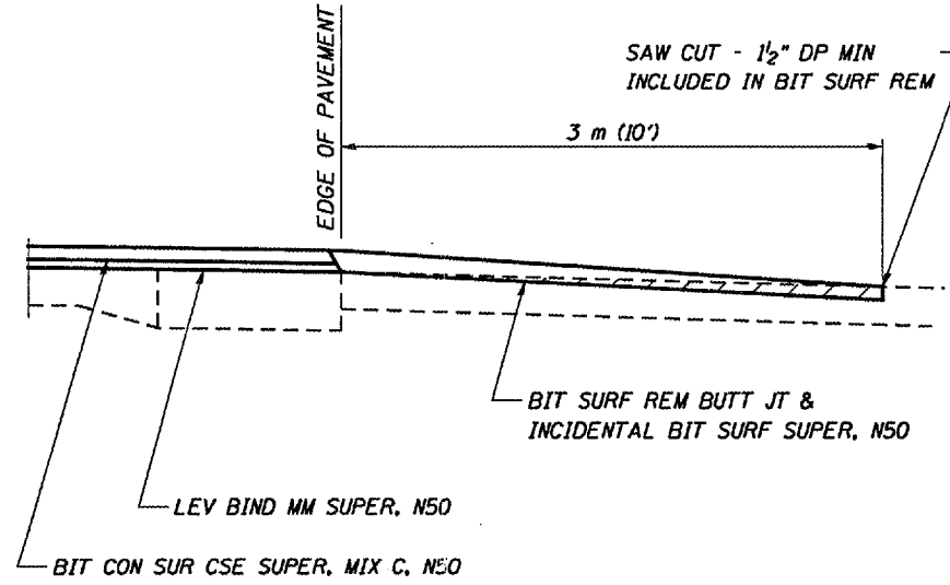
SECTION C-C FOR BITUMINOUS P.E., C.E.
