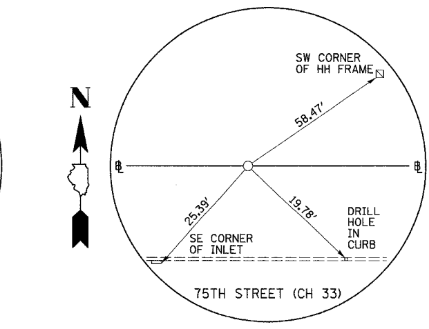
PI STA. 440+38.35 75TH STREET (CH 33) (5/8" I-ROD)
