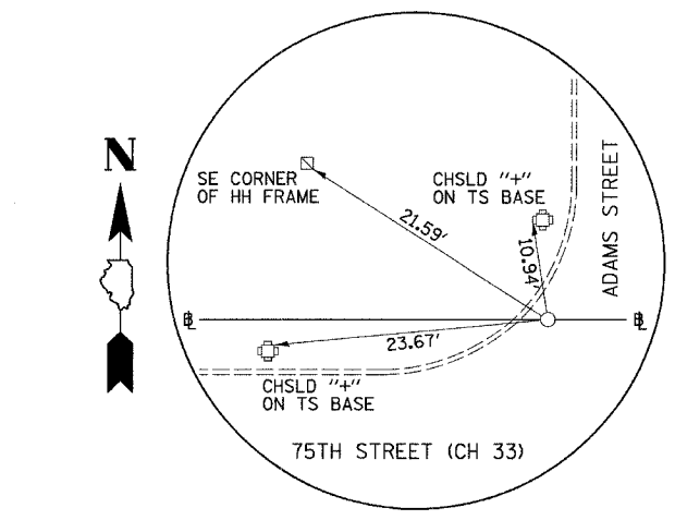
PI STA. 441+18.12 75TH STREET (CH 33) (PK NAIL)
