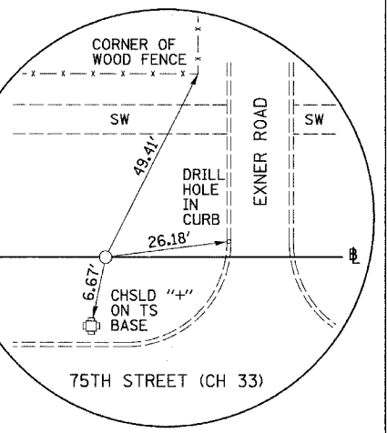
PI STA. 425+78.42 75TH STREET (CH 33) (5/8" I-ROD)
