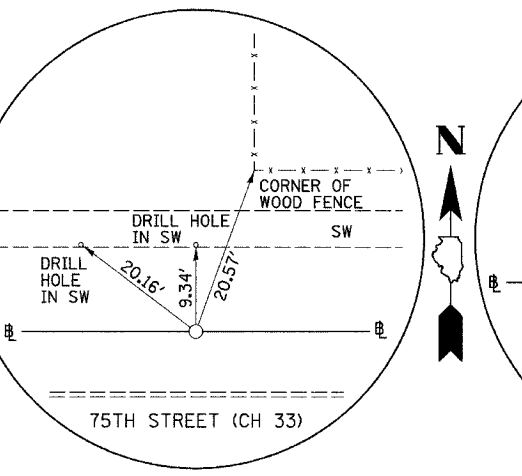
PI STA. 424+96.15 75TH STREET (CH 33) (5/8" I-ROD)
