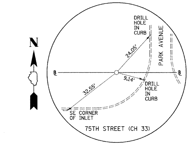
PI STA. 432+49.16 75TH STREET (CH 33) (5/8" I-ROD)
