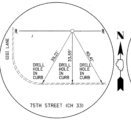
PI STA. 413+62.62 75TH STREET (CH 33) (5/8" I-ROD)
