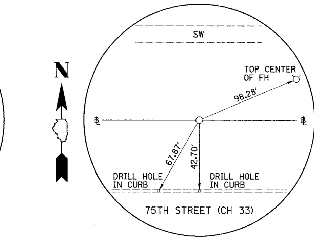
PI STA. 427+61.58 75TH STREET (CH 33) (5/8" I-ROD)
