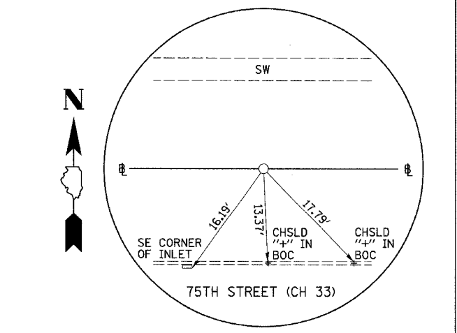
PI STA. 442+24.52 75TH STREET (CH 33) (5/8" I-ROD)
