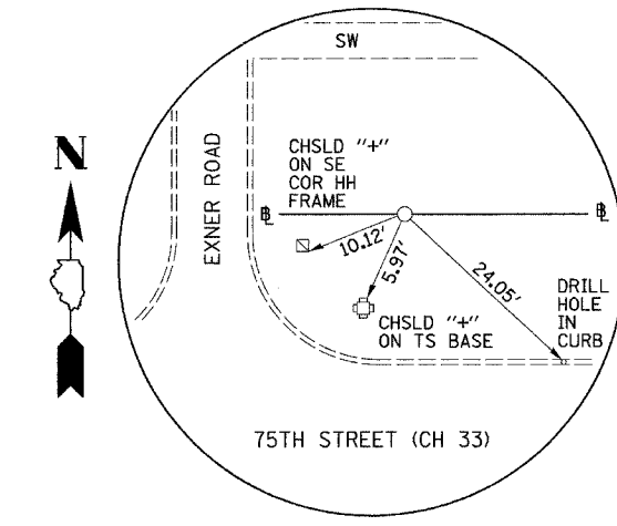
PI STA. 426+83.96 75TH STREET (CH 33) (5/8" I-ROD)
