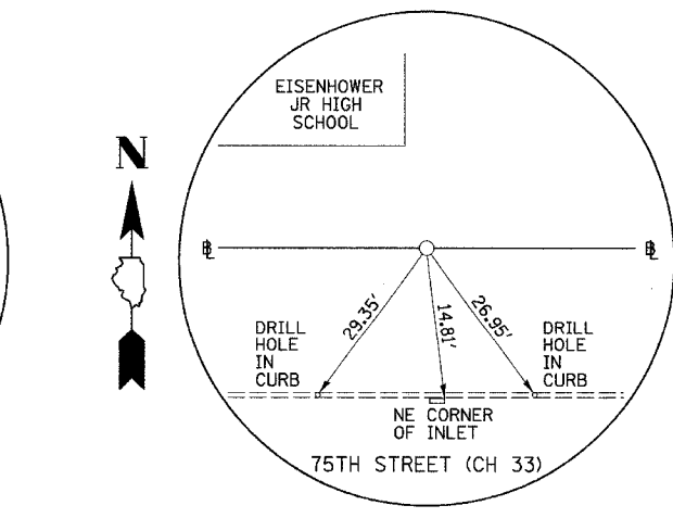
PI STA. 437+68.45 75TH STREET (CH 33) (5/8" I-ROD)
