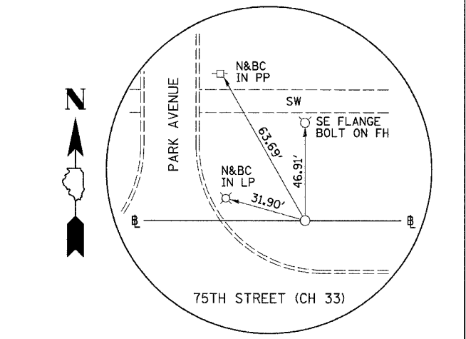
PI STA. 433+68.18 75TH STREET (CH 33) (5/8" I-ROD)
