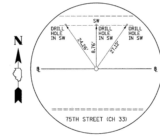
PI STA. 435+46.22 75TH STREET (CH 33) (5/8" I-ROD)
