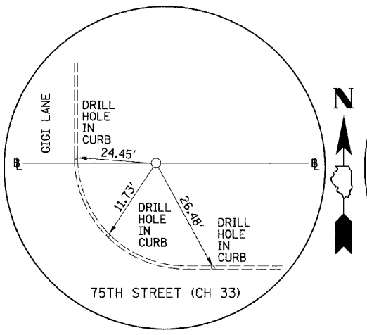
PI STA. 413+15.16 75TH STREET (CH 33) (5/8" I-ROD)
