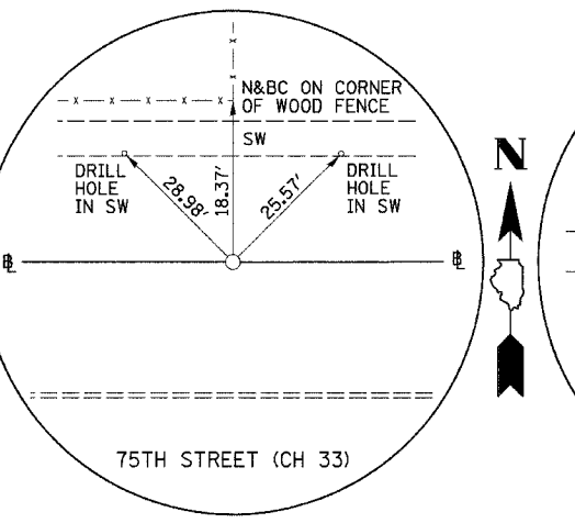
POT STA. 419+00.00 75TH STREET (CH 33) (5/8" I-ROD)
