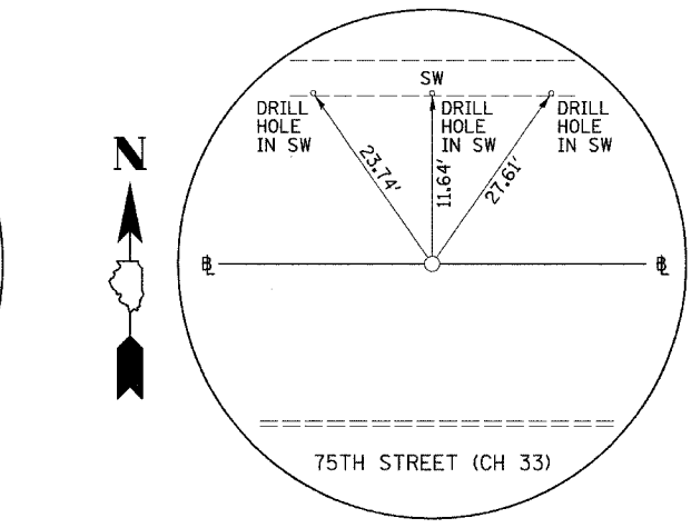
PI STA. 431+68.45 75TH STREET (CH 33) (5/8" I-ROD)
