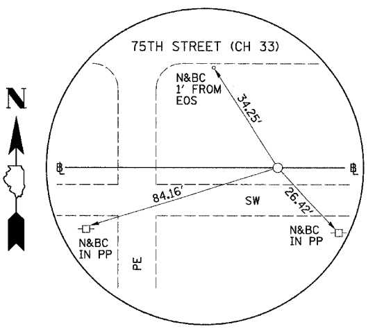
PI STA. 563+25.82 75TH STREET (CH 33) (5/8" I-ROD)
