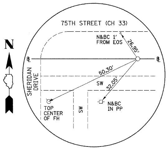
PI STA. 542+41.57 75TH STREET (CH 33) (5/8" I-ROD)
