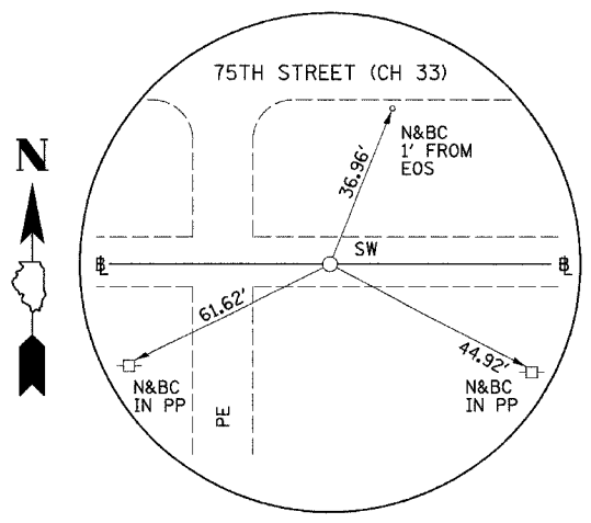
P.O.T. STA. 536+03.16 75TH STREET (CH 33) (CHSLD "+" ON SW)
