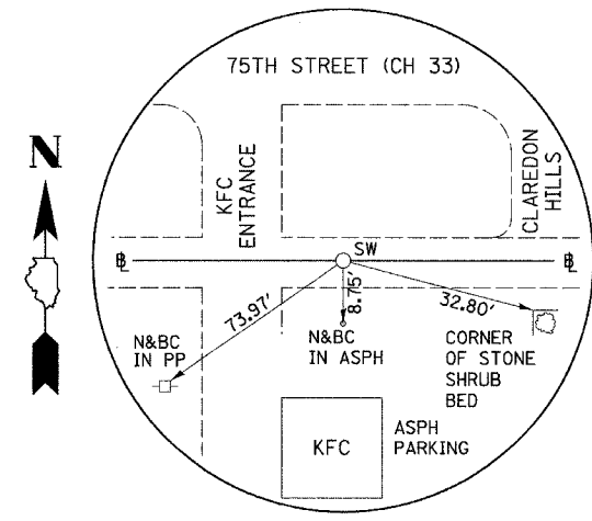
PI STA. 552+46.80 75TH STREET (CH 33) (5/8" I-ROD)
