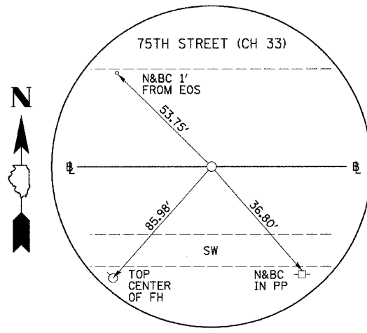
PI STA. 545+51.80 75TH STREET (CH 33) (5/8" I-ROD)
