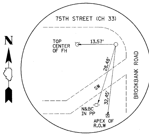
PI STA. 551+82.50 75TH STREET (CH 33) (5/8" I-ROD)
