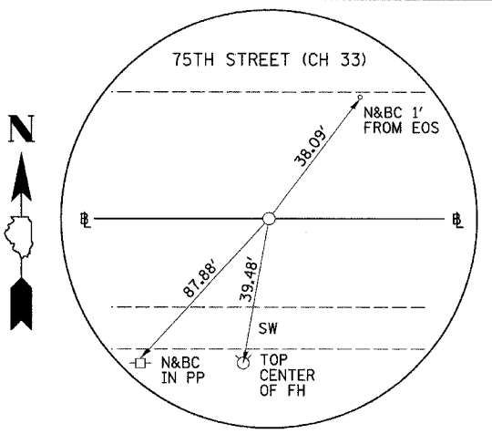
PI STA. 544+85.21 75TH STREET (CH 33) (5/8" I-ROD)
