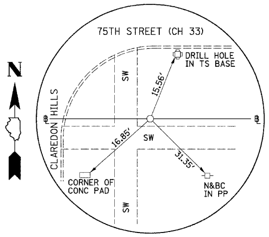
PI STA. 553+94.35 75TH STREET (CH 33) (5/8" I-ROD)
