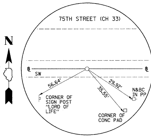
PI STA. 539+92.38 75TH STREET (CH 33) (CHSLD "+" ON SW)
