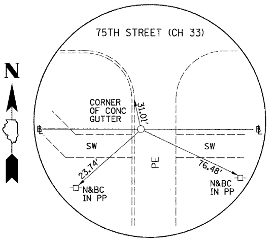
PI STA. 555+08.91 75TH STREET (CH 33) (PK NAIL IN PVMT)
