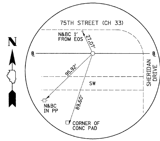
PI STA. 541+13.92 75TH STREET (CH 33) (5/8" I-ROD)
