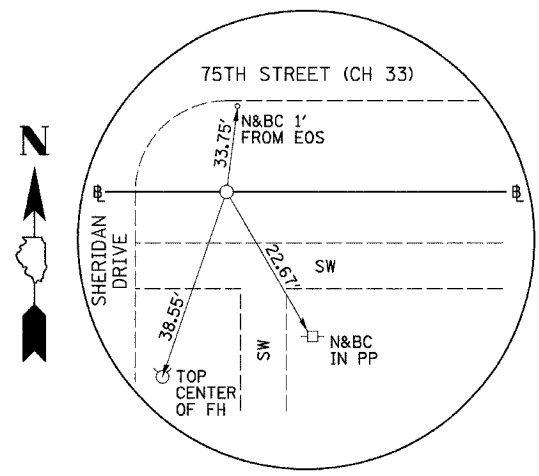
PI STA. 542+10.55 75TH STREET (CH 33) (5/8" I-ROD)
