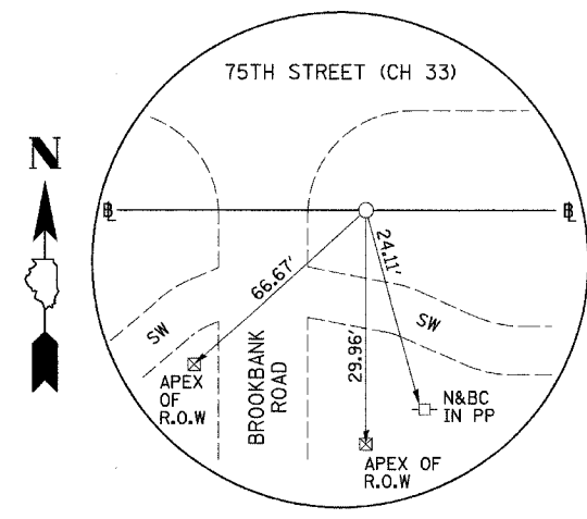
PI STA. 558+25.37 75TH STREET (CH 33) (5/8" I-ROD)
