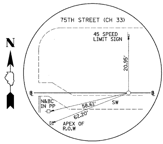
PI STA. 558+91.54 75TH STREET (CH 33) (5/8" I-ROD)
