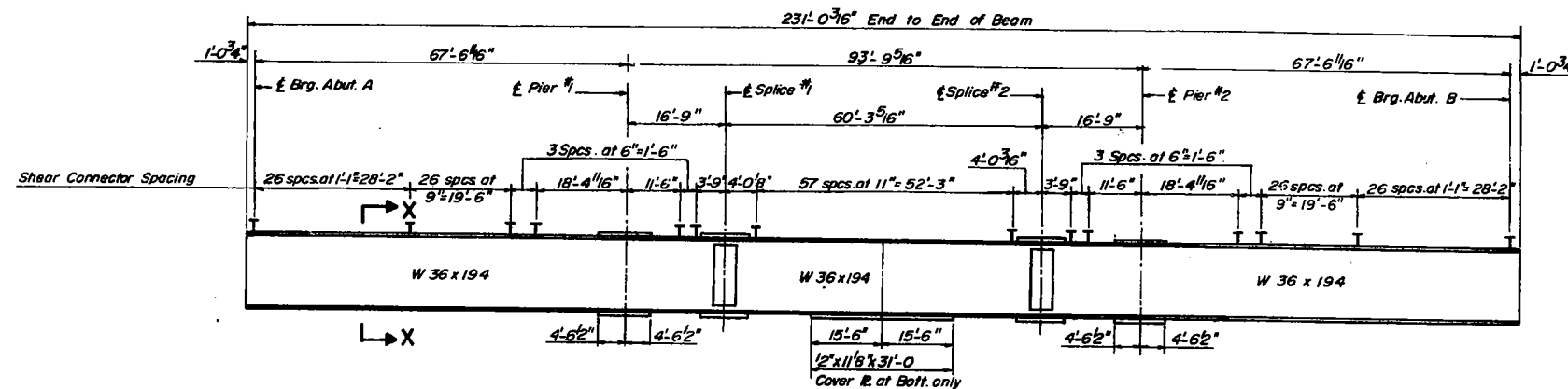
BEAM ELEVATION WEST BOUND (TYP)
