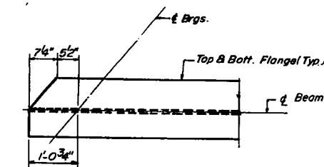
TYPICAL BEAM END
