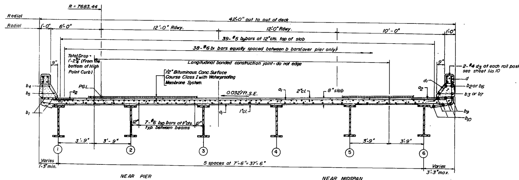
CROSS SECTION Looking Ahead Station
