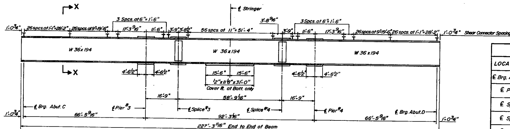
BEAM ELEVATION EAST BOUND (TYP)
