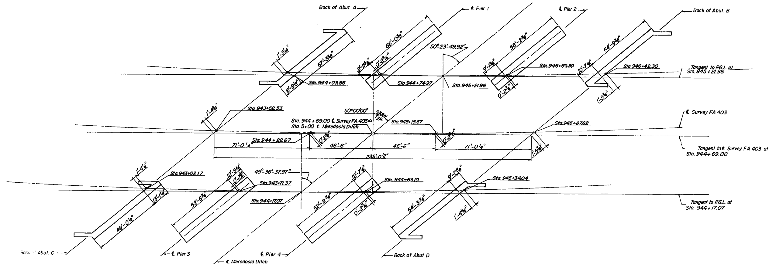
FOOTING LAYOUT
