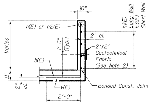
SECTION C-C (Long Wall Similar)
