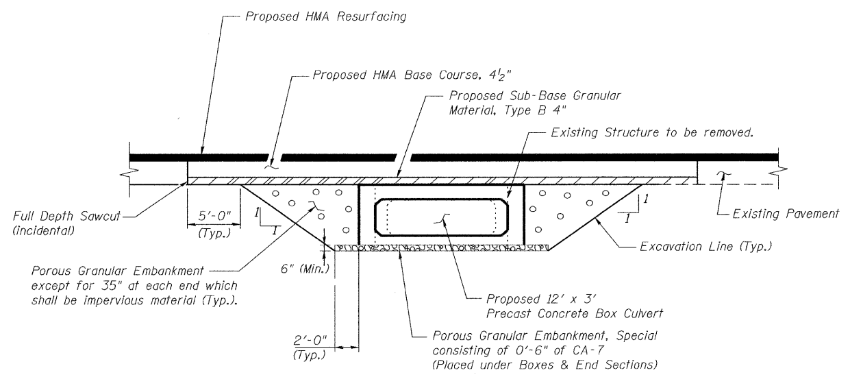
SECTION THROUGH PRECAST BOX CULVERT
