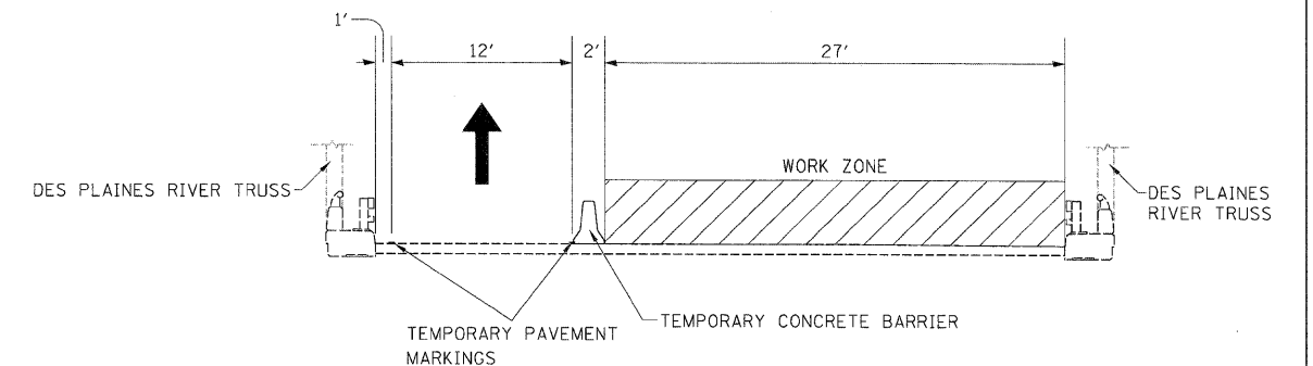
STAGE 1 CONSTRUCTION FOR WB I-80 OVER DES PLAINES RIVER, BNSF RAILROAD/GARDNER STREET, AND HICKORY CREEK LOOKING WEST
