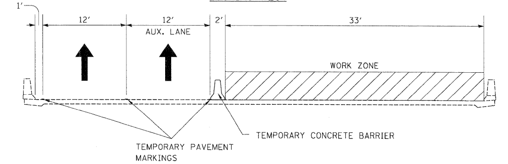
STAGE 2 CONSTRUCTION FOR WB I-80 OVER DES PLAINES RIVER, BNSF RAILROAD/GARDNER STREET, AND HICKORY CREEK LOOKING WEST
