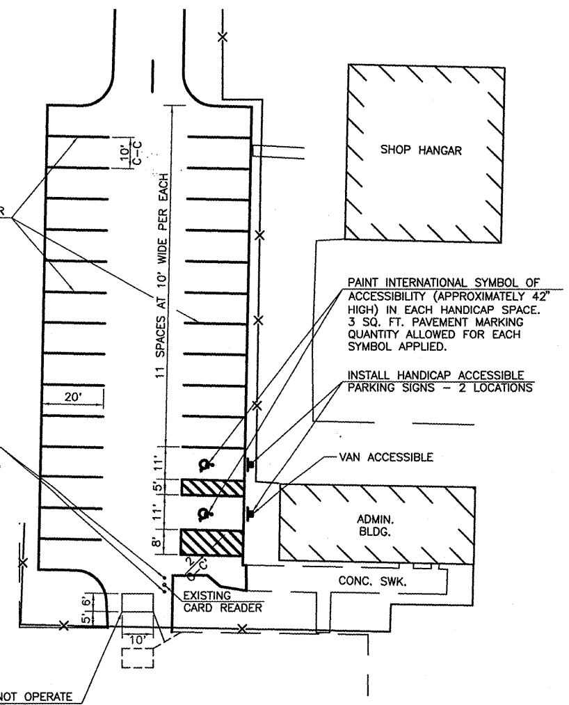
DETAIL 'A' GRAPHIC SCALE IN FEET (0, 20, 40)
