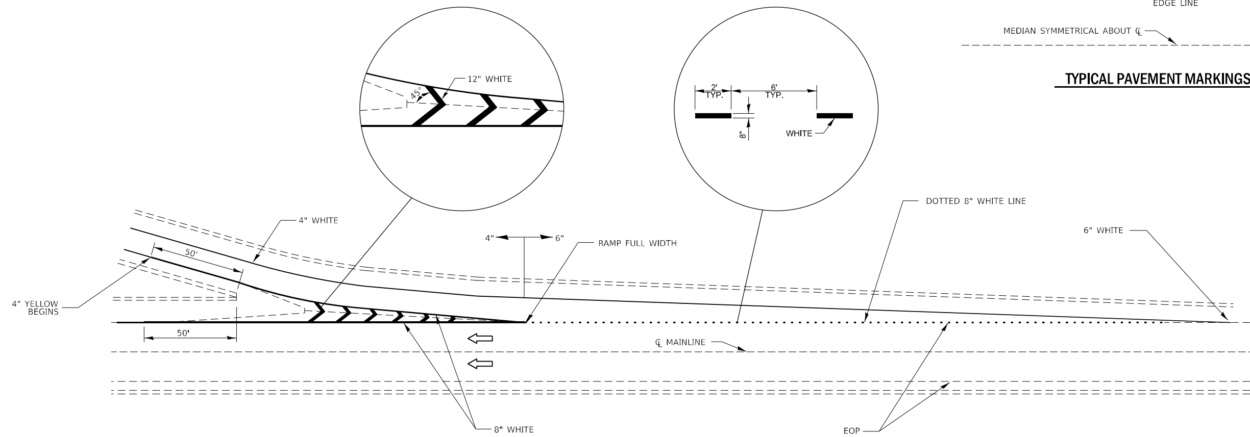
TYPICAL PAVEMENT MARKINGS FOR EXIT RAMP TERMINALS
