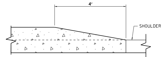
DETAIL OF CURB HEIGHT TRANSITION
