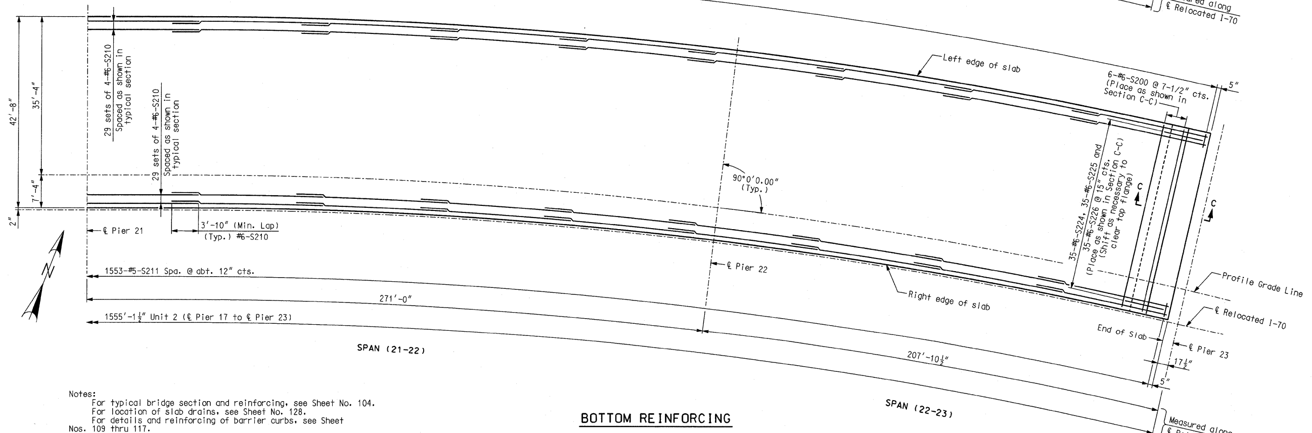
SLAB PLAN SHOWING REINFORCING WB - UNIT 2 (3 OF 3)
