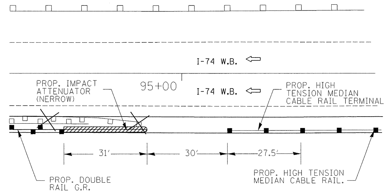
CABLE GUARD WITH IMPACT ATTENUATOR
