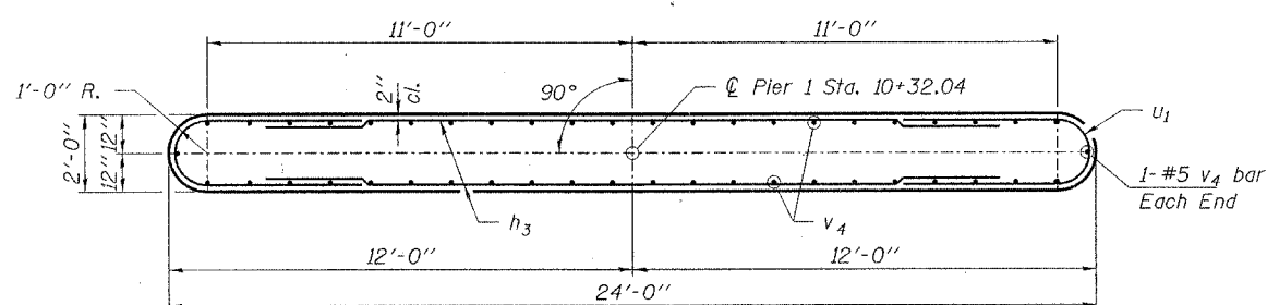
SECTION B-B
