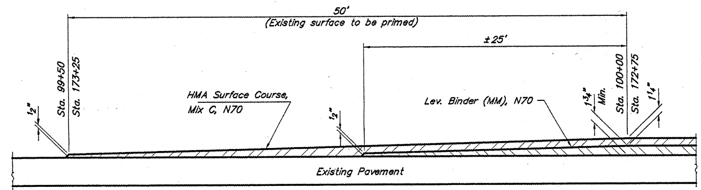
BEGINNING & ENDING TAPER
