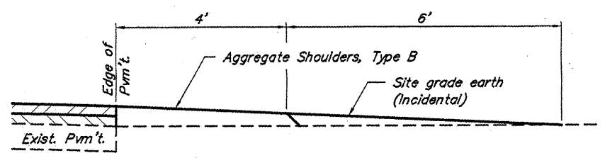
SECTION A-A FIELD ENTRANCE (Est. No. = 3)
