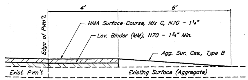
SECTION A-A PRIVATE ENTRANCE - AGGREGATE (Est. No. = 4)
