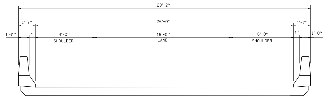
TYPICAL SECTION
