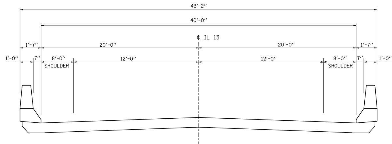
TYPICAL SECTION
