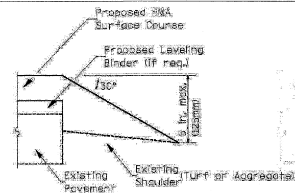
SECTION A-A RURAL MAILBOX TURNOUT DETAILS
