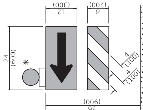
DIRECTION INDICATOR BARRICADE
