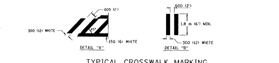
TYPICAL CROSSWALK MARKING
