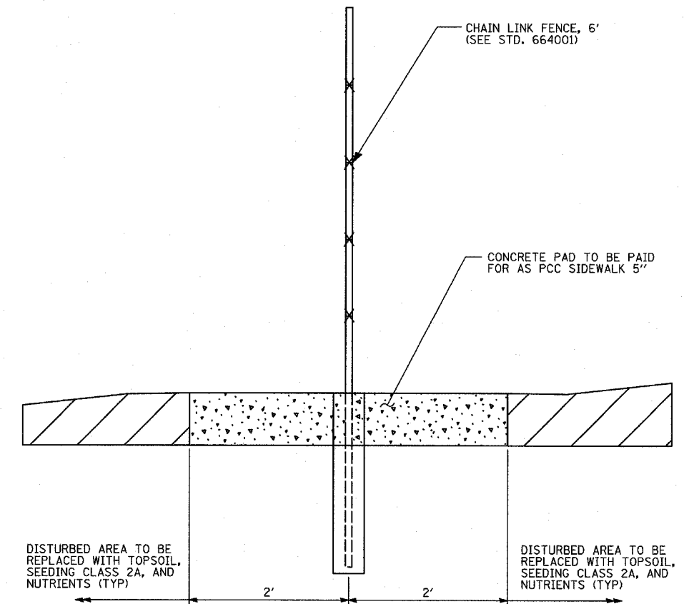
FENCE MOUNTED ON CONCRETE PAD
