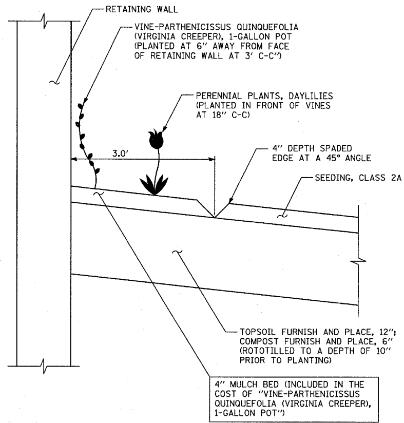
VINE AND DAYLILY PLANTING DETAIL
