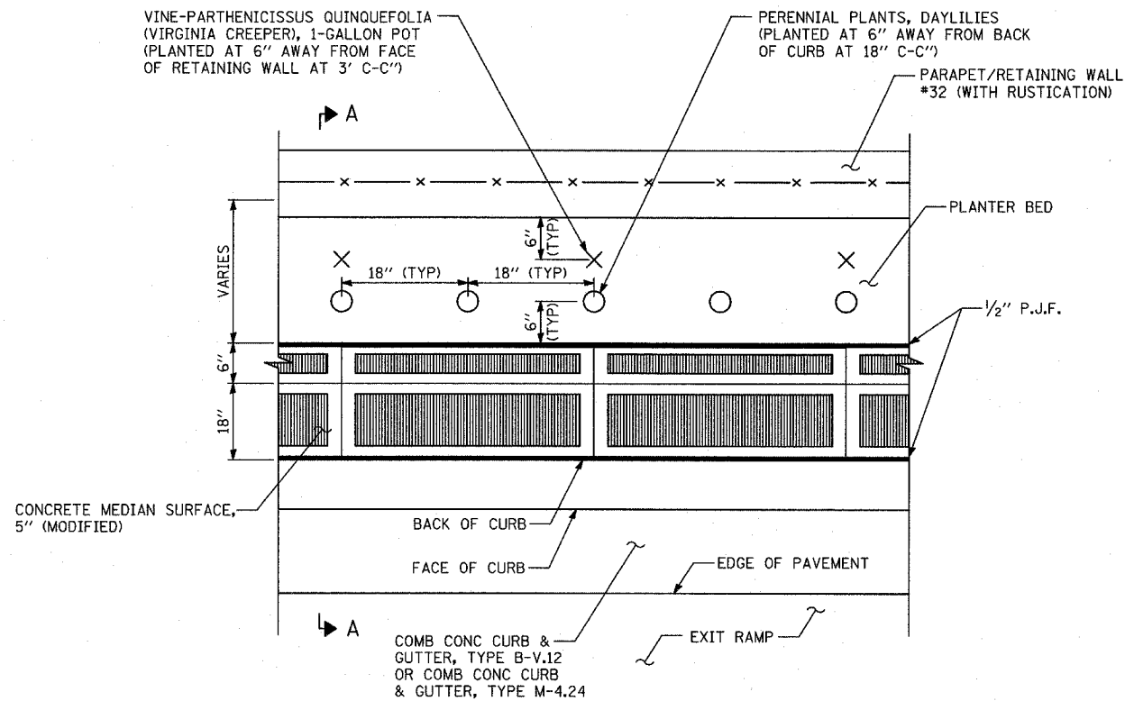
PLANTER BED - WALL #68 AT WENTWORTH AVENUE EXIT RAMP
