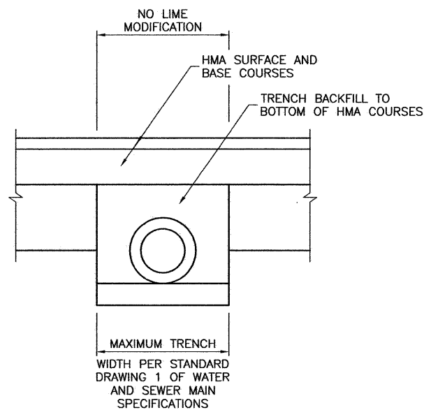
BACKFILL DETAIL
