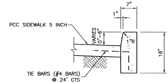
BARRIER CURB ADJACENT TO PCC SIDEWALK 5 INCH
