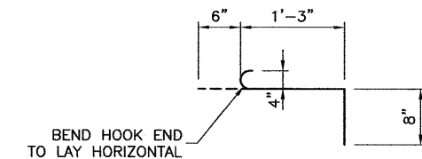
TIE BAR (#4 BARS) TIE BARS WILL BE PAID FOR EACH
