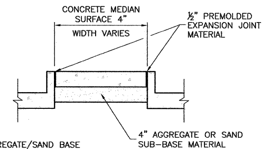
CONCRETE MEDIAN SURFACE, 4 INCH
