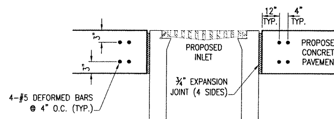
STRUCTURE PAVEMENT REINFORCING FOR INLET "NOT TO SCALE"
