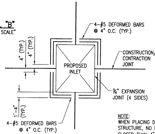
STRUCTURE PAVEMENT REINFORCING FOR INLET "NOT TO SCALE"
