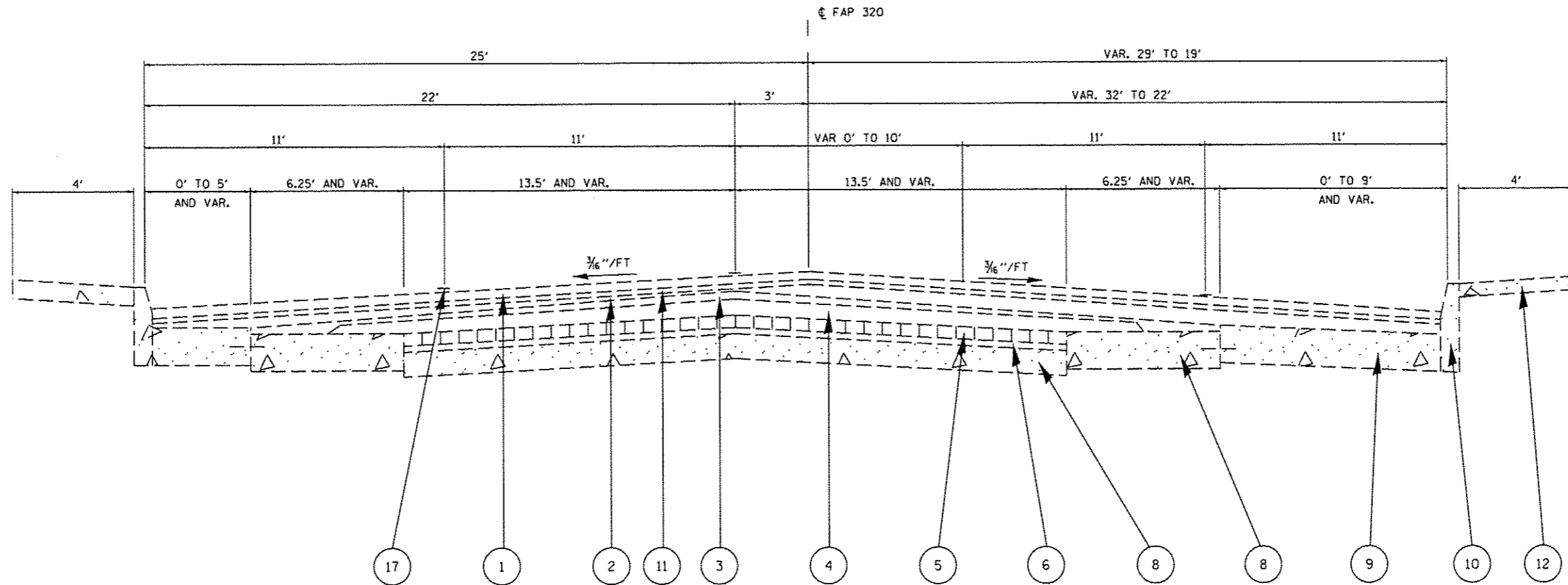
TYPICAL #4
