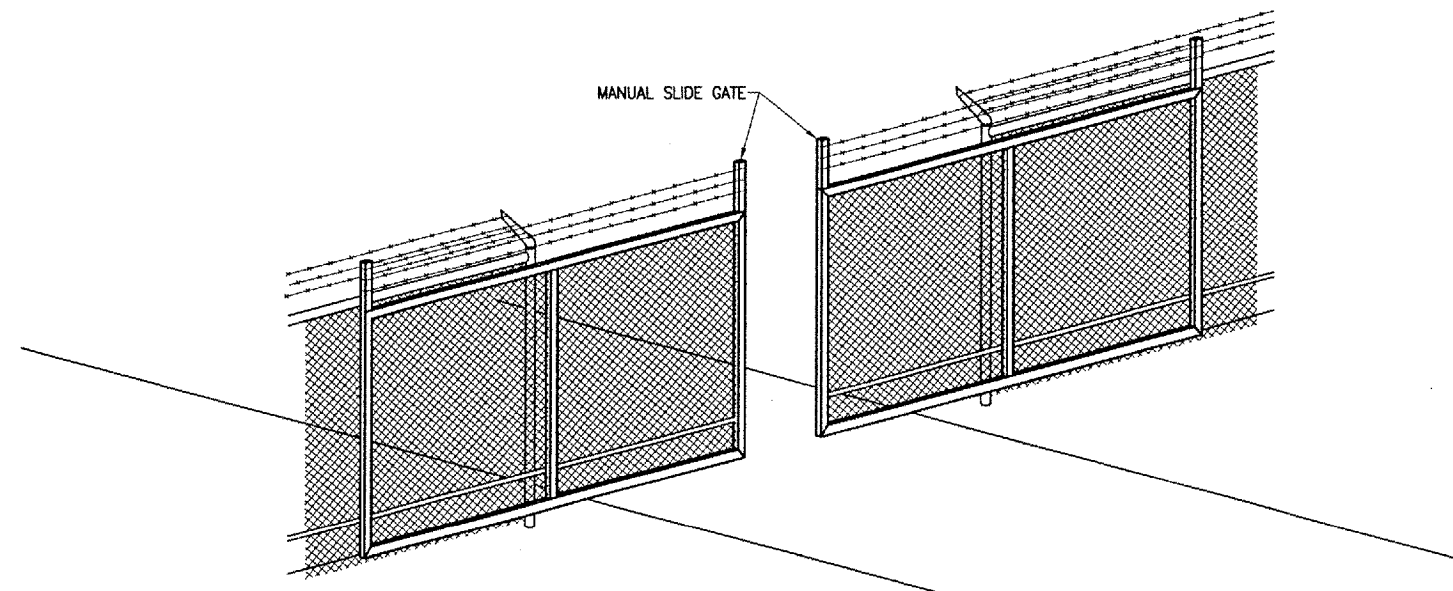
MANUAL SLIDE GATE DETAIL "NOT TO SCALE"
