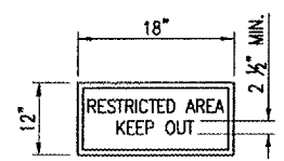
SIGN DETAIL "NOT TO SCALE"
