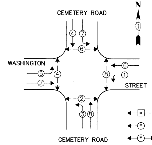
TEMPORARY CONTROLLER SEQUENCE STAGE 3 & 4
