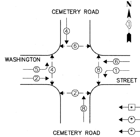
TEMPORARY CONTROLLER SEQUENCE STAGE 1 & 2
