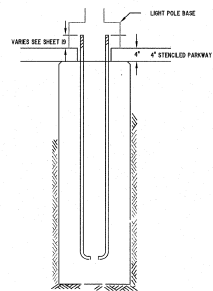
LIGHT POLE FOUNDATION & MOUNTING DETAIL
