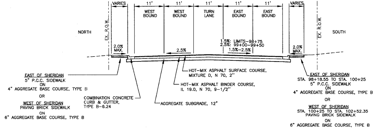
PROPOSED TYPICAL SECTION GRAND AVENUE STA. 98+18.55 TO STA. 102+52.35
