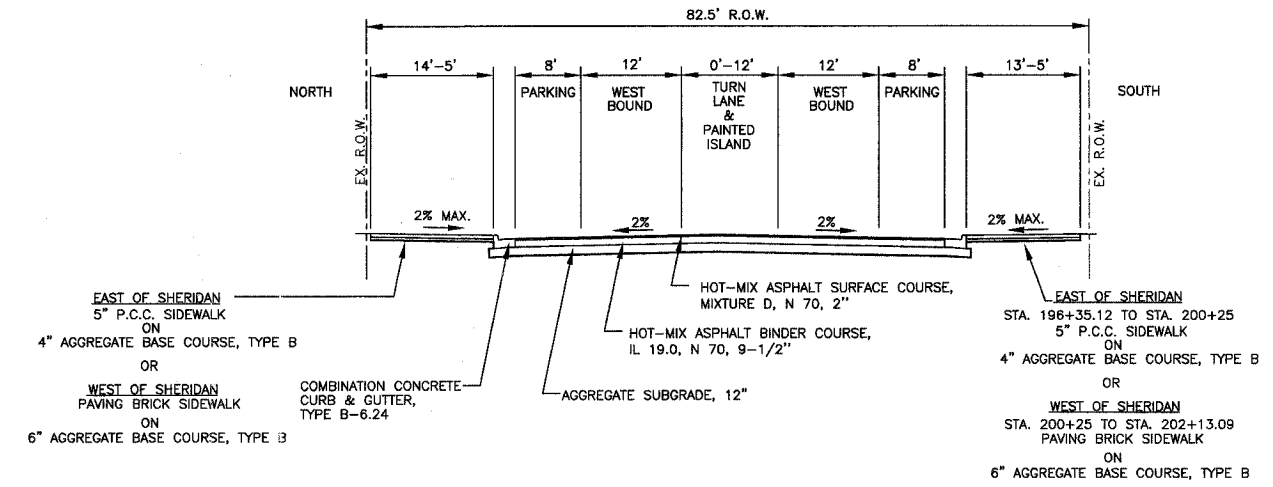
PROPOSED TYPICAL SECTION WASHINGTON STREET STA. 198+35.12 TO STA. 202+13.09
