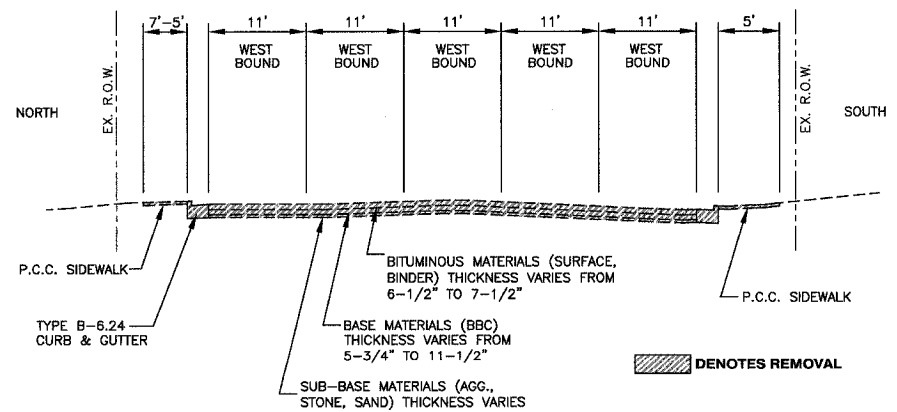
EXISTING TYPICAL SECTION GRAND AVENUE STA. 98+18.55 TO STA. 102+52.35
