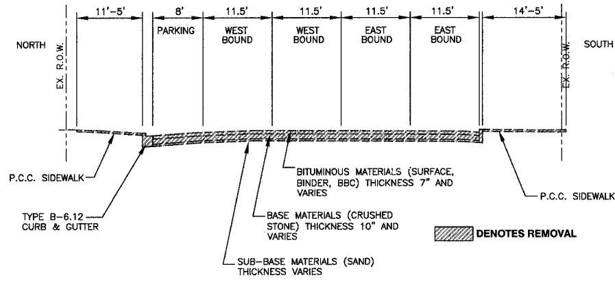
EXISTING TYPICAL SECTION WASHINGTON STREET STA. 198+35.12 TO STA. 202+13.09
