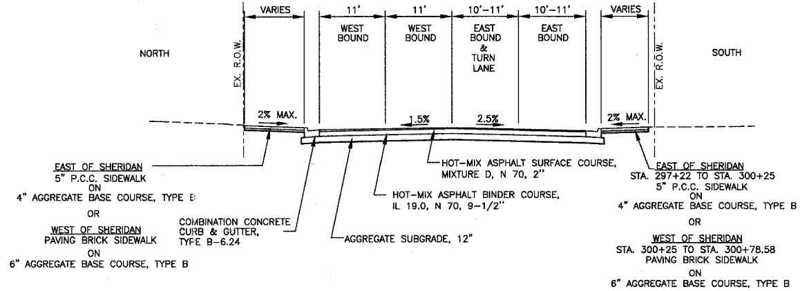
PROPOSED TYPICAL SECTION BELVIDERE ROAD STA. 297+22 TO STA. 300+78.58
