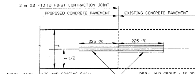
JOINT DETAIL AT CONTRACT TERMINAL(S)
