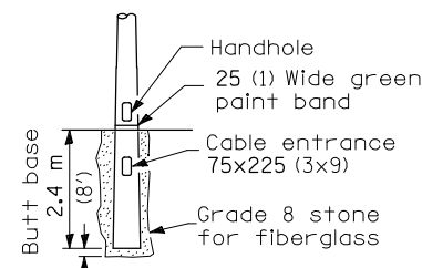
BUTT BASE
