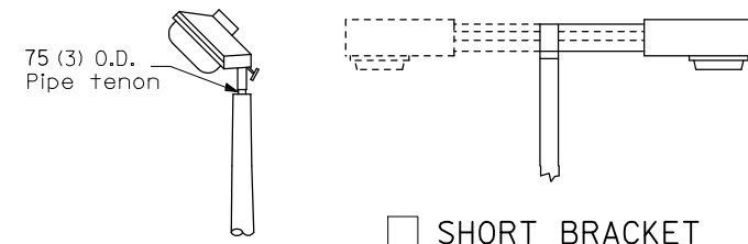
TENON
