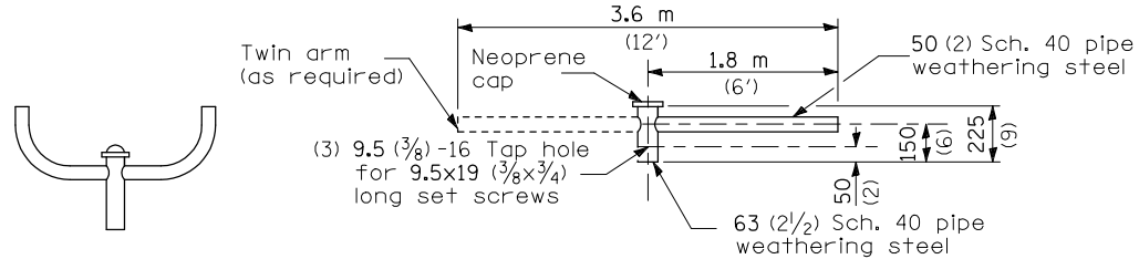
TWIN TENON
