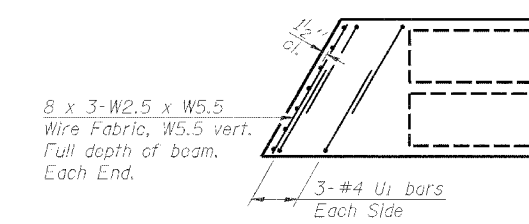
END PLAN
