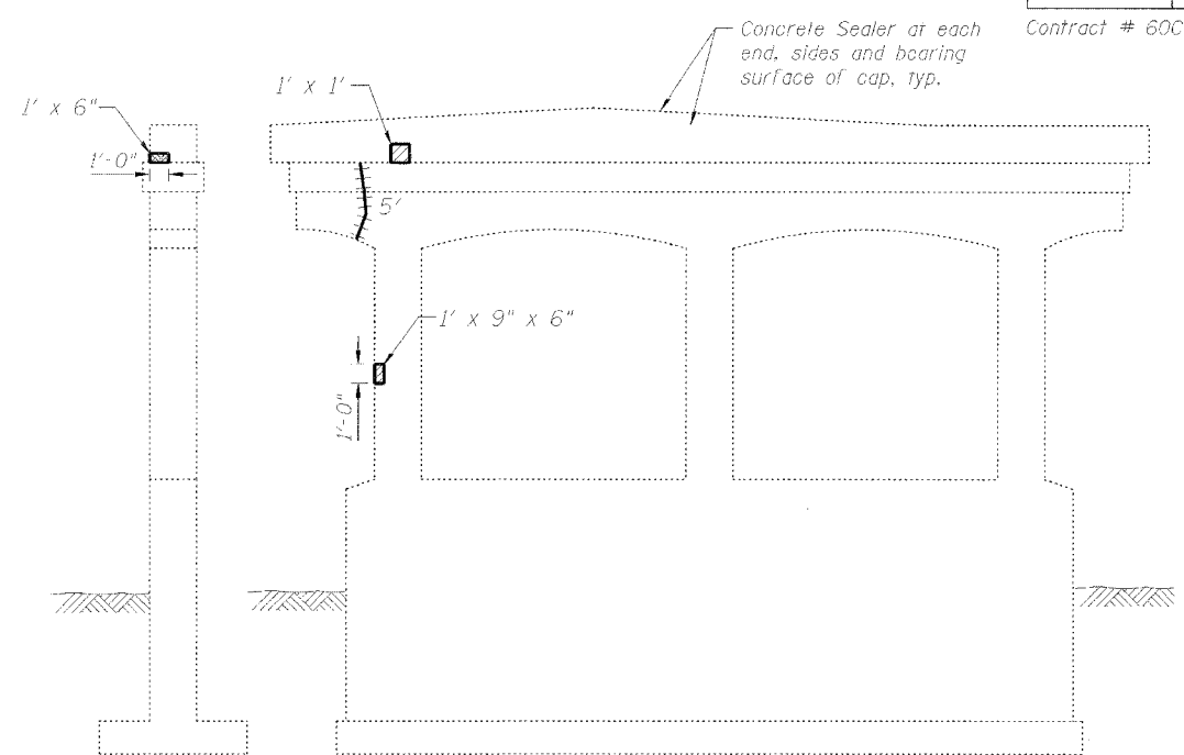
EAST ELEVATION
