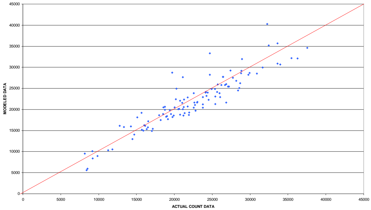
COMPARISON OF MODELED VS ACTUAL COUNT DATA ON ARTERIALS - ALL DAY VOLUME
