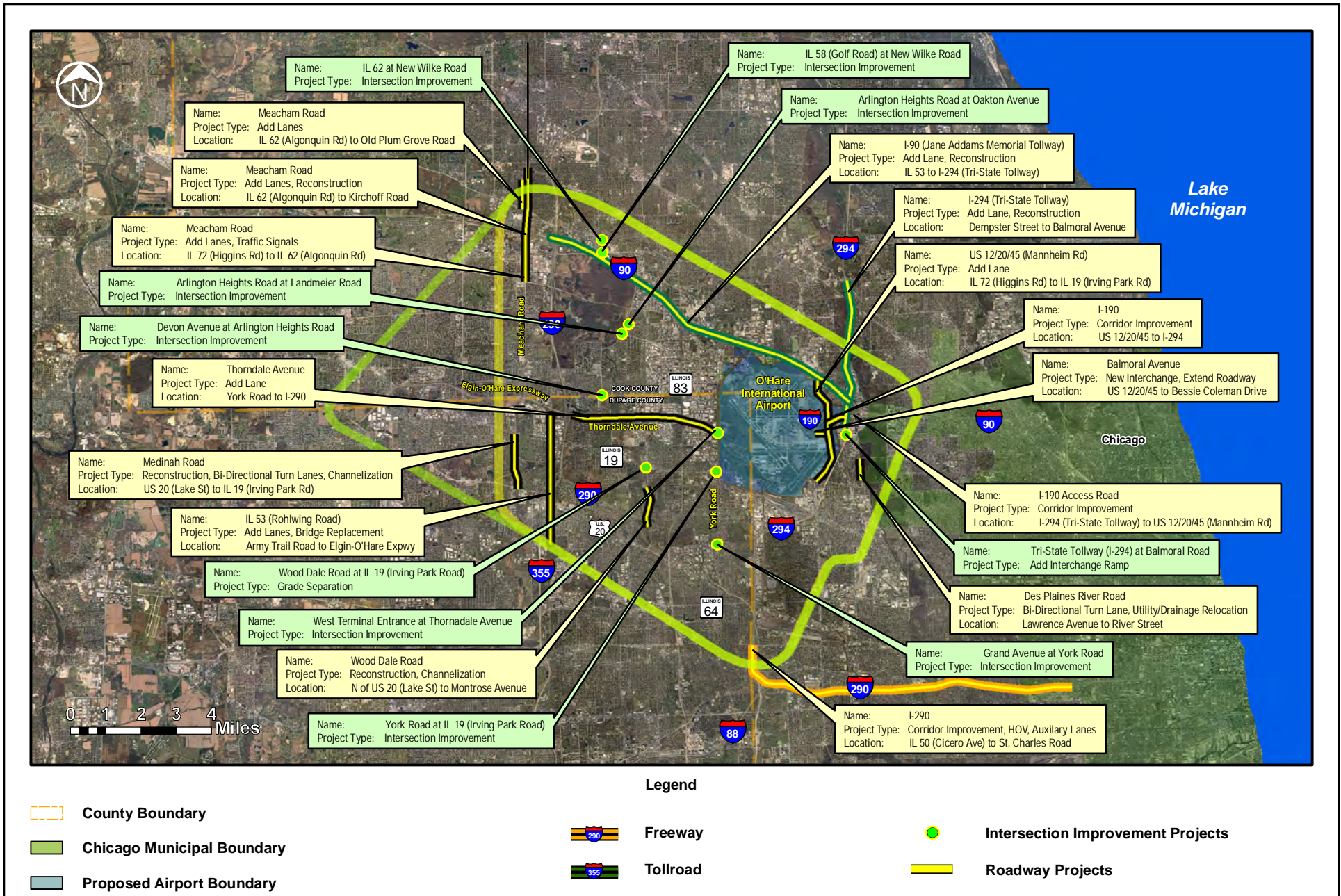
Elgin O'Hare - West Bypass 2030 Baseline - Roadway Project Map Exhibit 4-1
