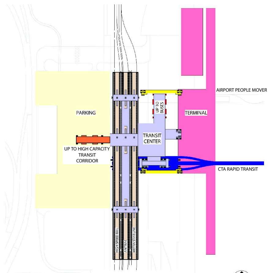
Schematic Plan Below Grade
