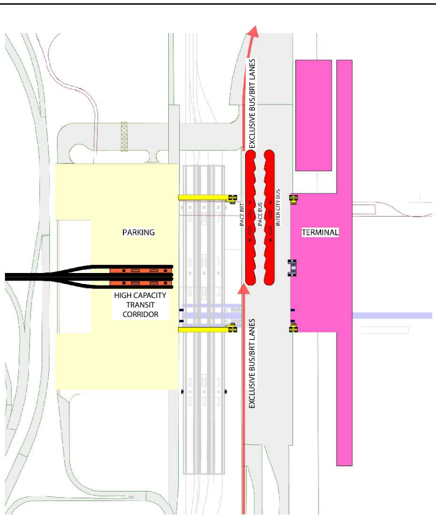
Schematic Plan at Grade
