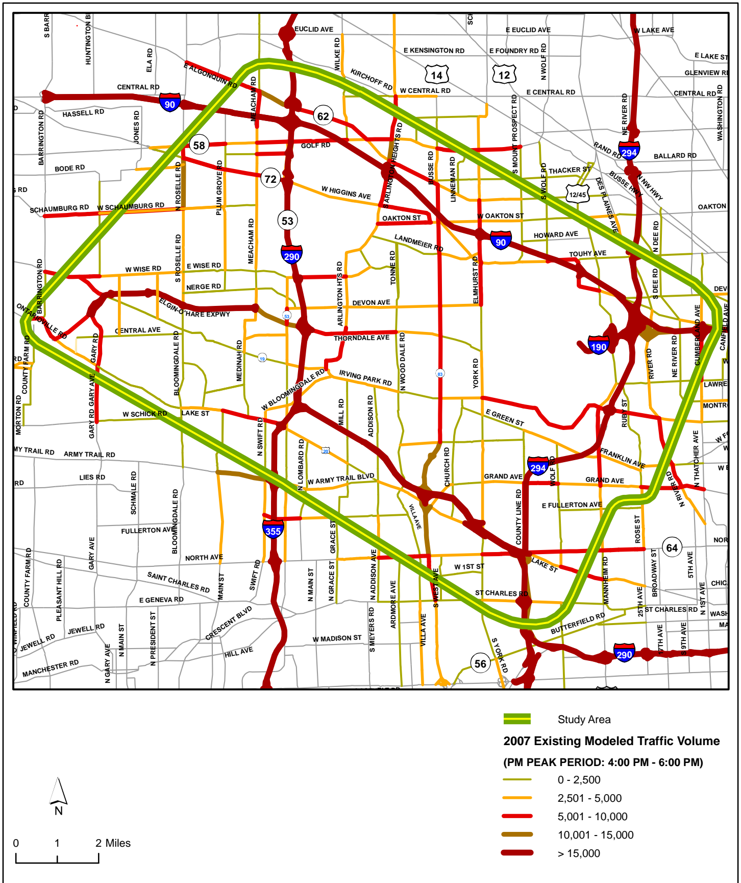
Elgin O'Hare - West Bypass 2007 P.M. Peak Period Modeled Traffic Volume in Revised Study Area Exhibit 3-3A
