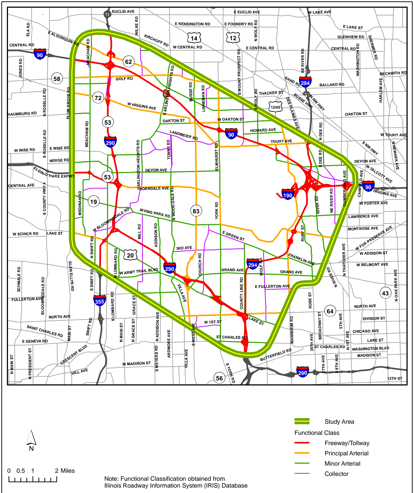
Elgin O'Hare - West Bypass Functional Classification of Roadways in the Study Area Exhibit 3-2
