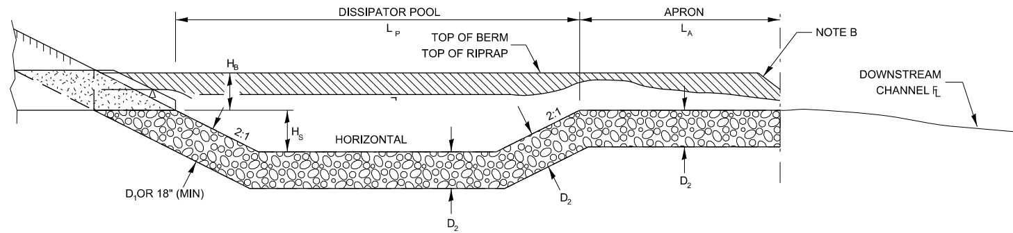
SECTION
