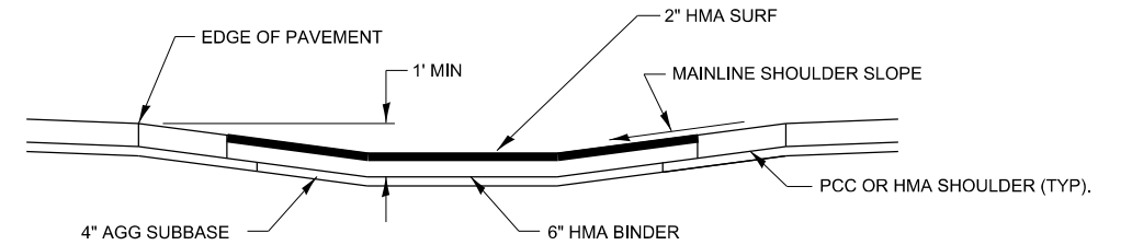
SECTION B-B
