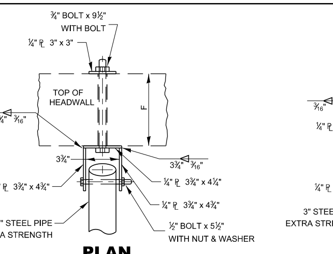
PLAN HEADWALL BRACKET ASSEMBLY
