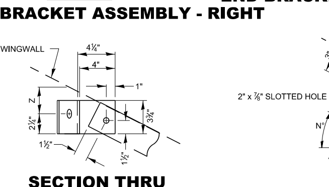
SECTION THRU DETAIL D
