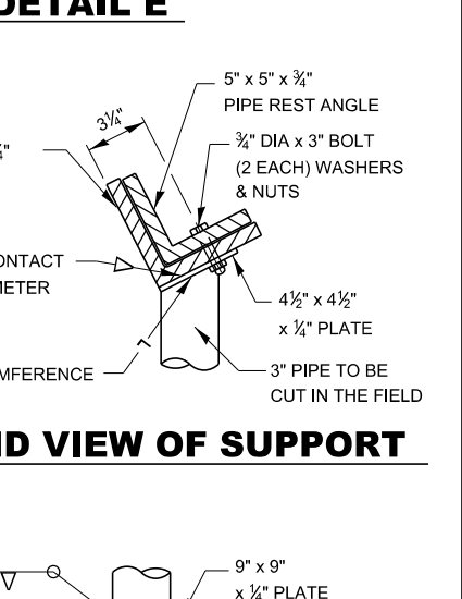
END VIEW OF SUPPORT
