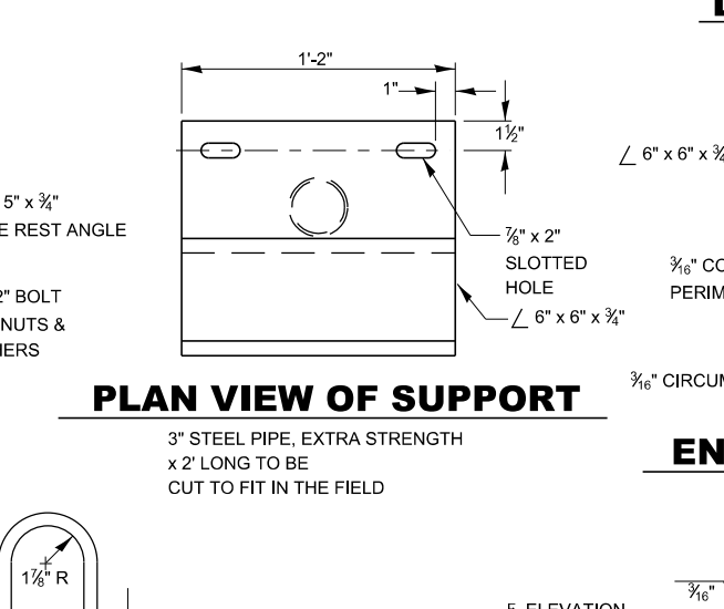
PLAN VIEW OF SUPPORT
