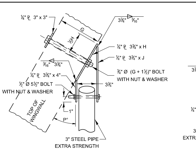
PLAN WINGWALL BRACKET ASSEMBLY - LEFT
