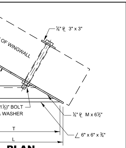
PLAN END BRACKET ASSEMBLY - RIGHT
