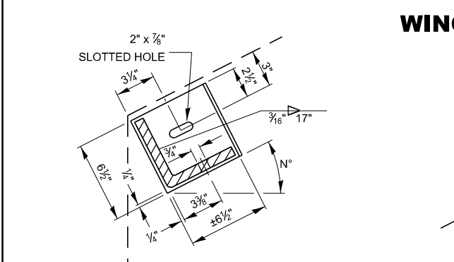
SECTION THRU DETAIL A
