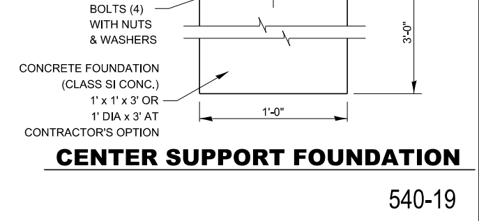
CENTER SUPPORT FOUNDATION
