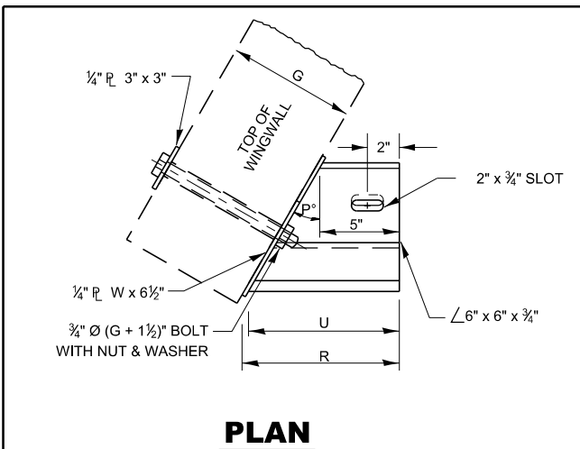
PLAN END BRACKET ASSEMBLY - LEFT
