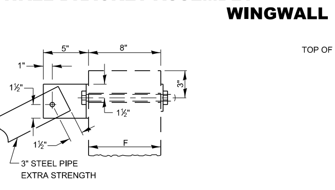
SECTION THRU DETAIL C
